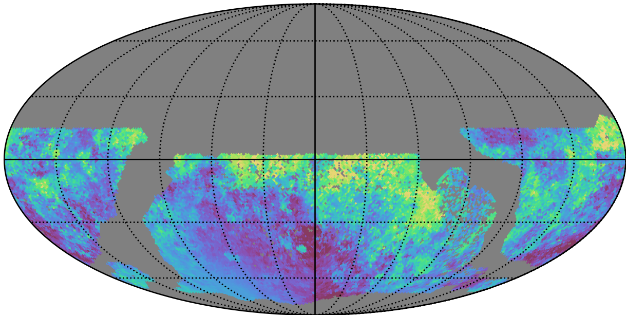
no_high_blob_v3.3_10yrs WFD i band: Median moonDistance
