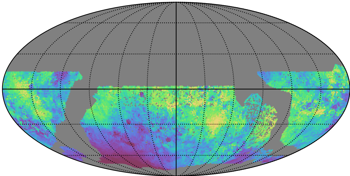
no_high_blob_v3.3_10yrs WFD g band: Median moonDistance
