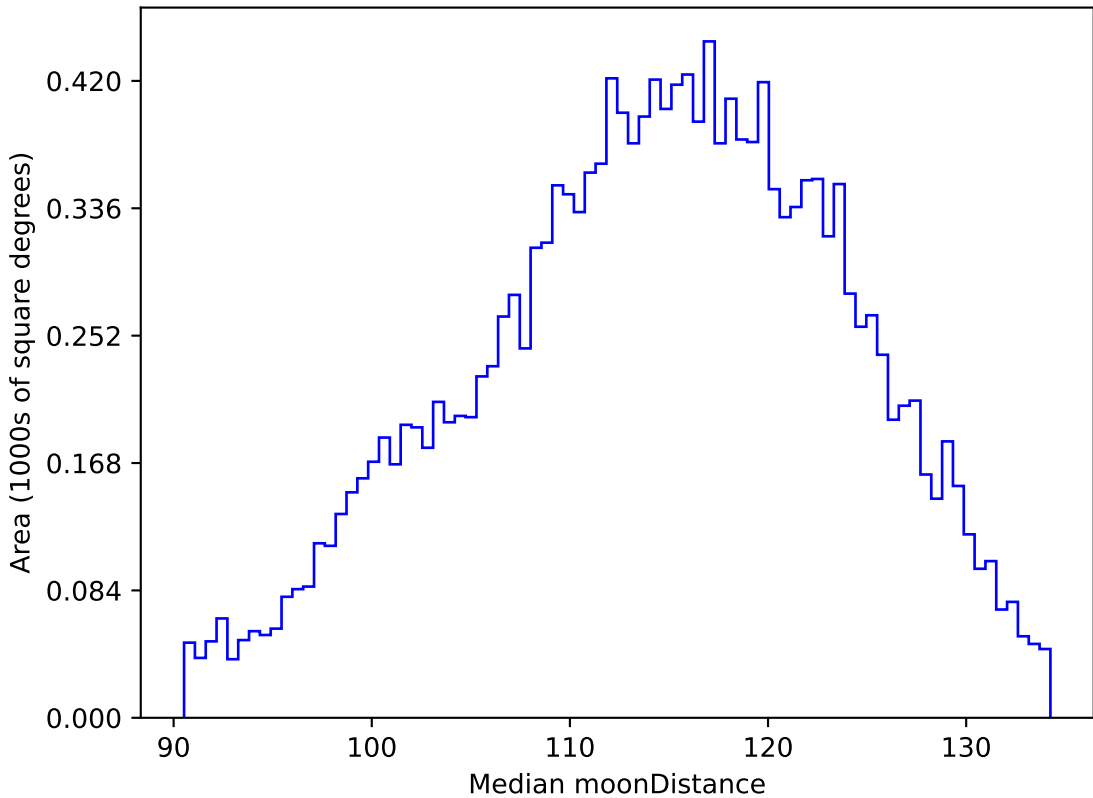
no_high_blob_v3.3_10yrs WFD g band: Median moonDistance
