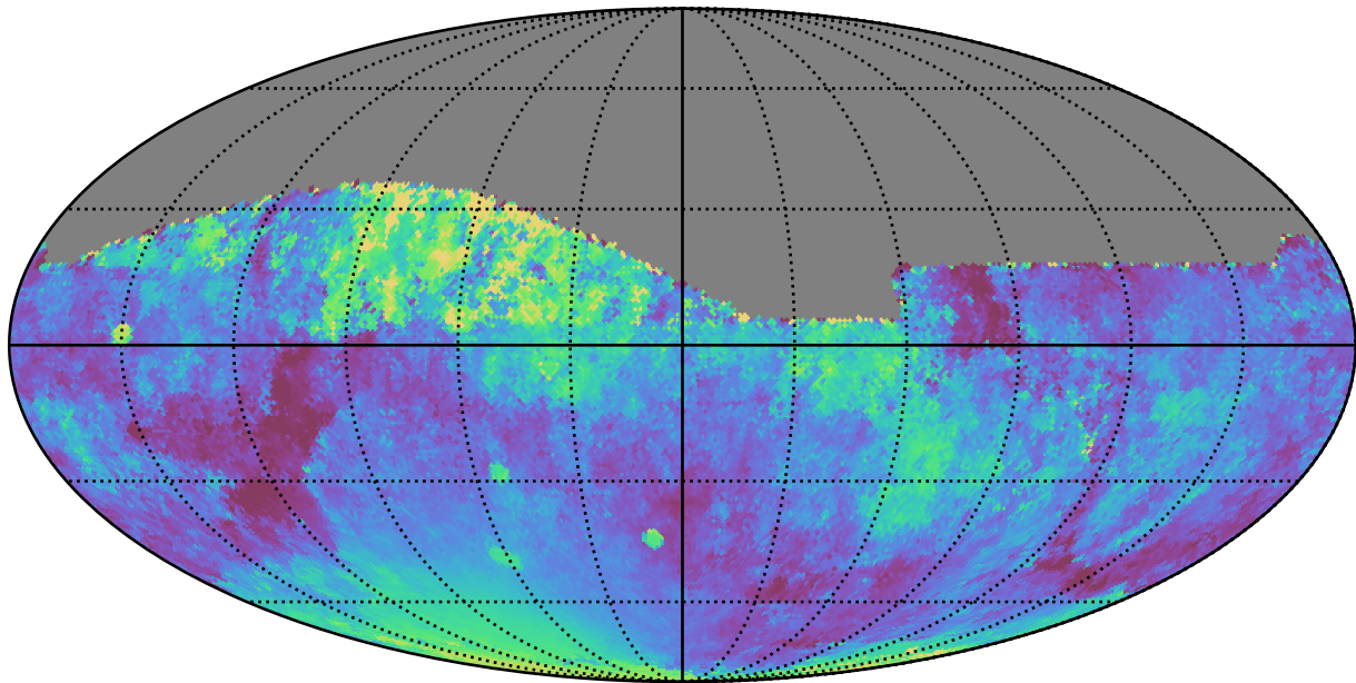
no_high_blob_v3.3_10yrs All sky z band: Median moonDistance
