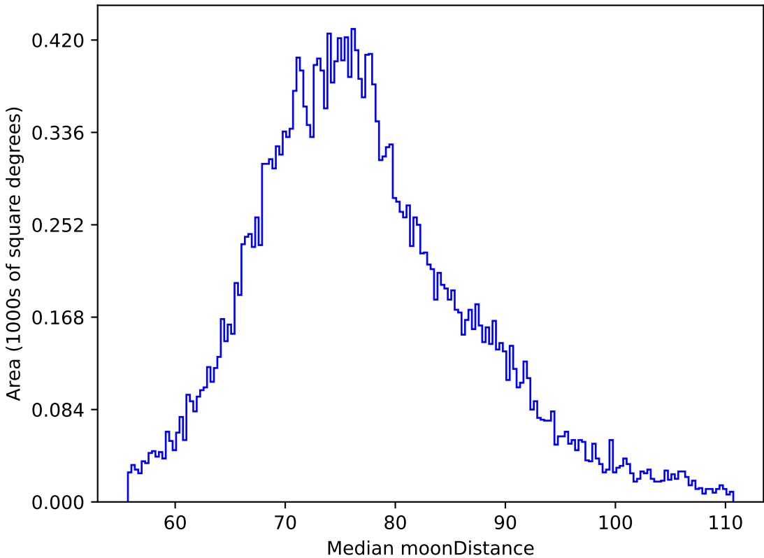
no_high_blob_v3.3_10yrs All sky z band: Median moonDistance
