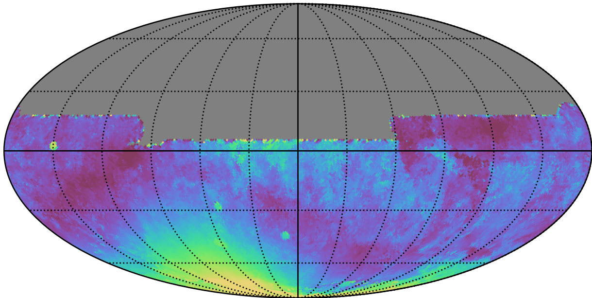
no_high_blob_v3.3_10yrs All sky y band: Median moonDistance
