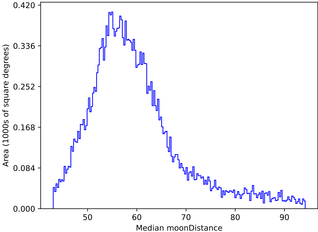
no_high_blob_v3.3_10yrs All sky y band: Median moonDistance
