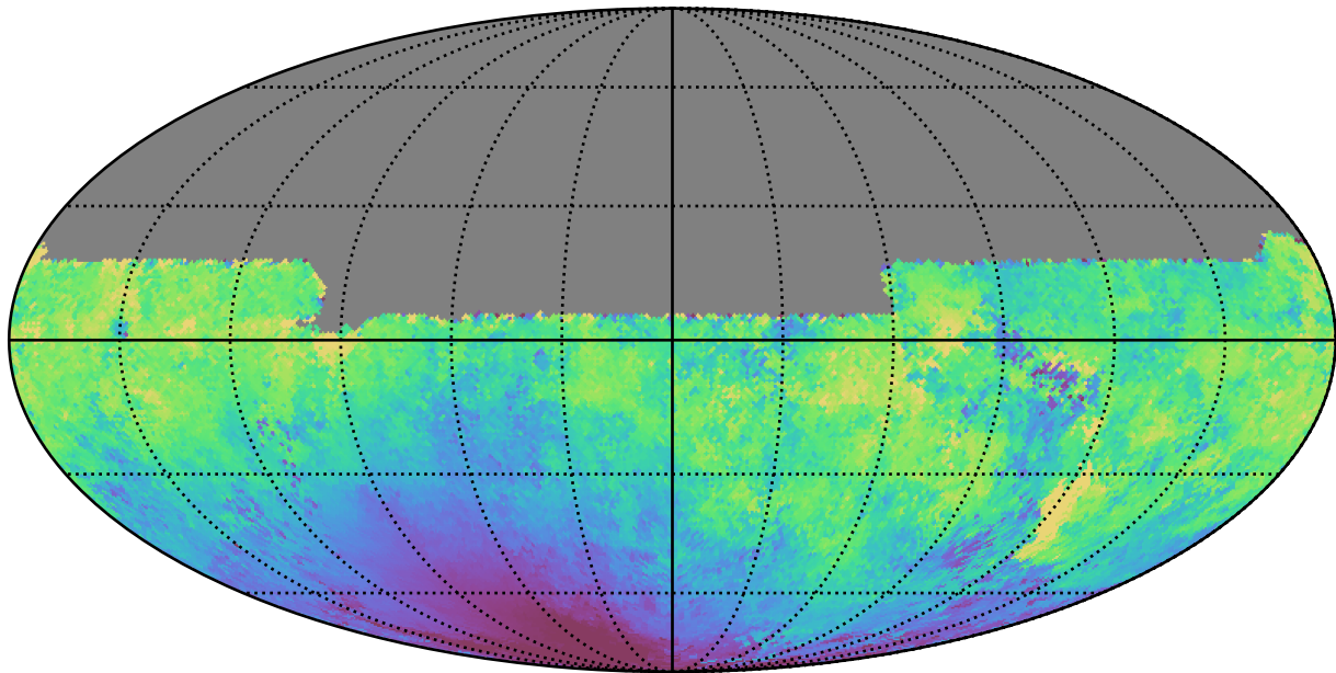
no_high_blob_v3.3_10yrs All sky u band: Median moonDistance
