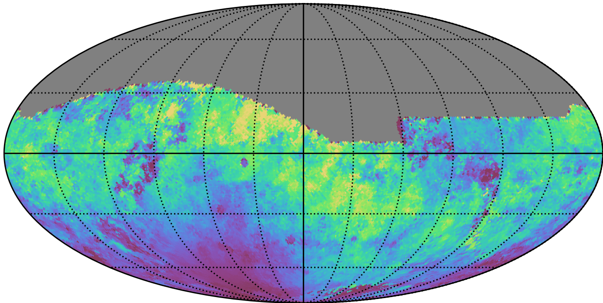
no_high_blob_v3.3_10yrs All sky r band: Median moonDistance
