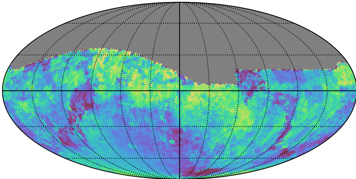
no_high_blob_v3.3_10yrs All sky i band: Median moonDistance
