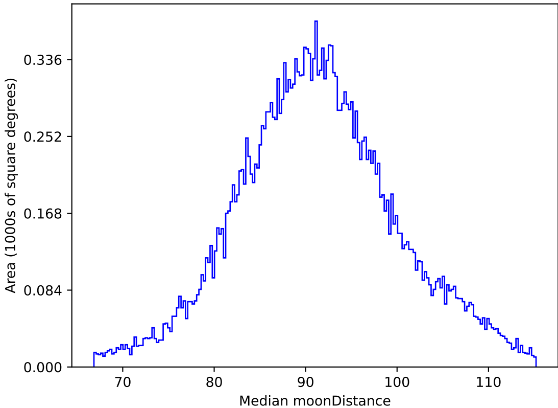
no_high_blob_v3.3_10yrs All sky i band: Median moonDistance
