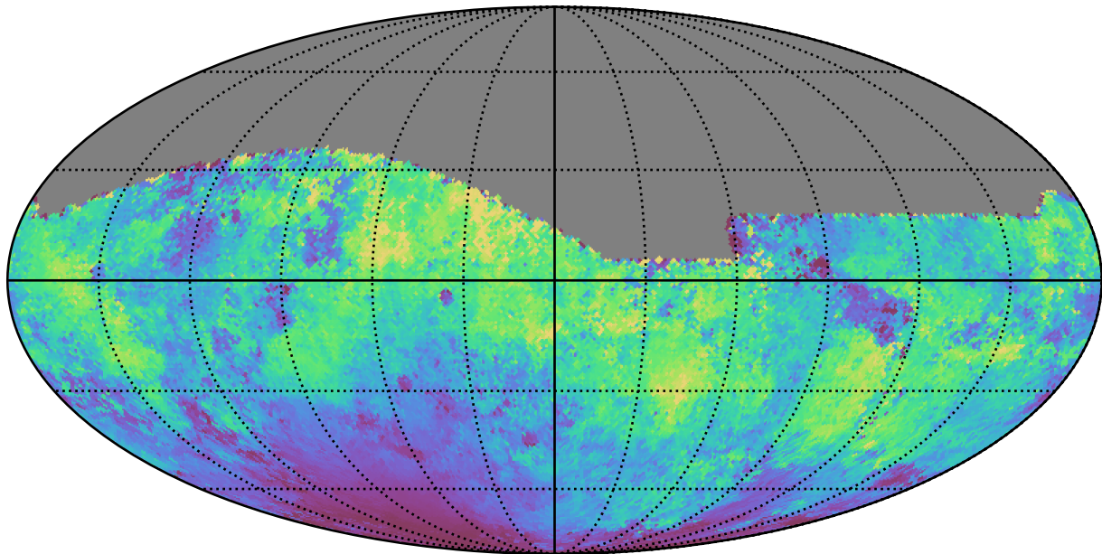
no_high_blob_v3.3_10yrs All sky g band: Median moonDistance
