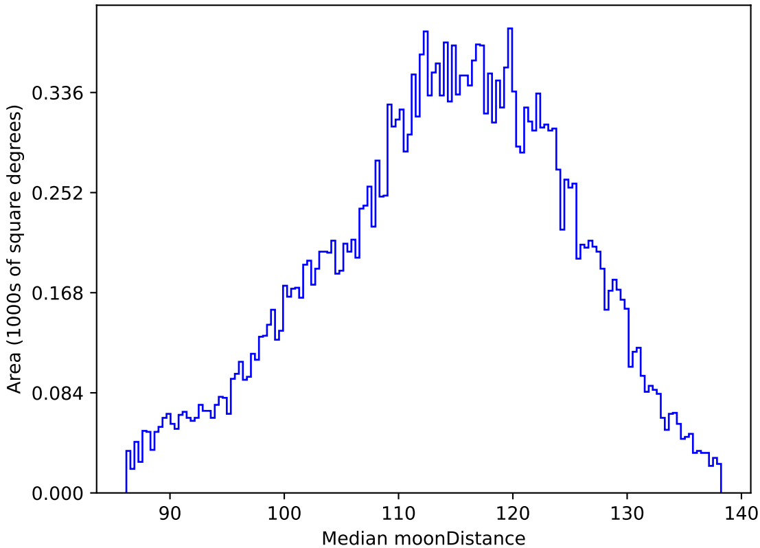
no_high_blob_v3.3_10yrs All sky g band: Median moonDistance
