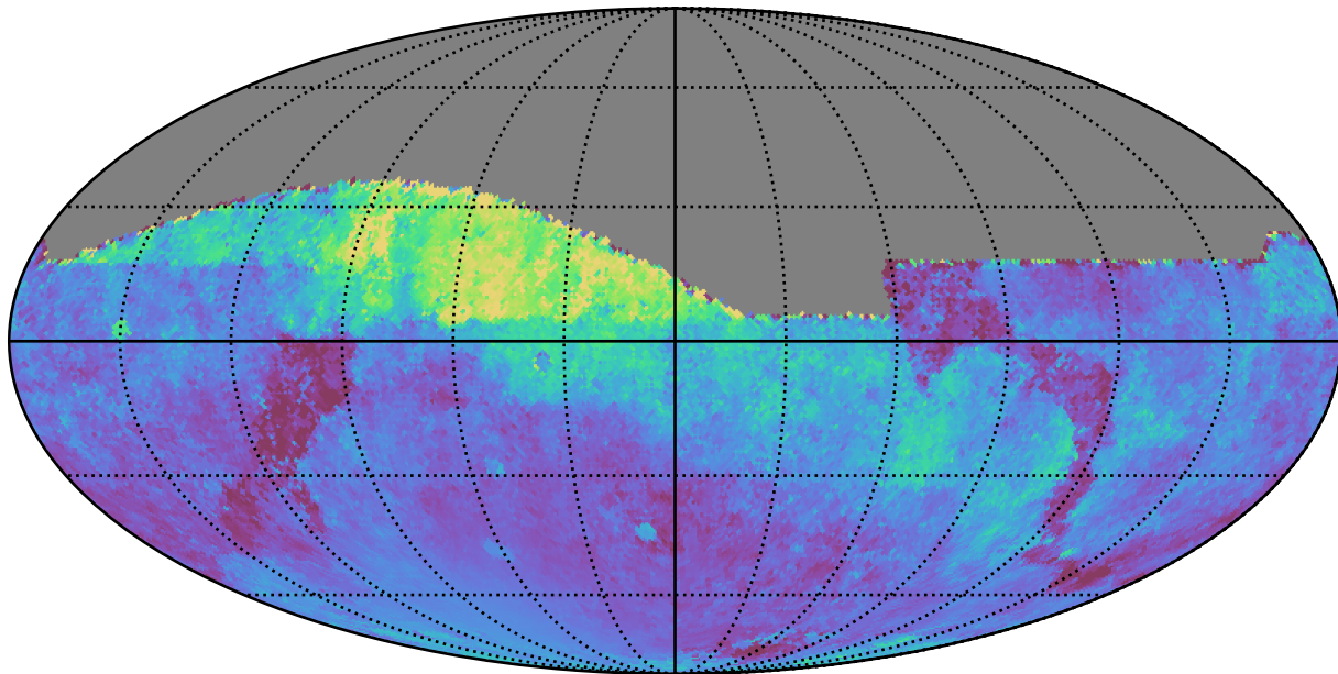
no_high_blob_v3.3_10yrs All sky all bands: Median moonDistance
