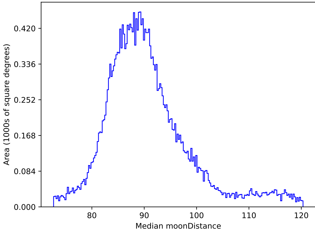
no_high_blob_v3.3_10yrs All sky all bands: Median moonDistance
