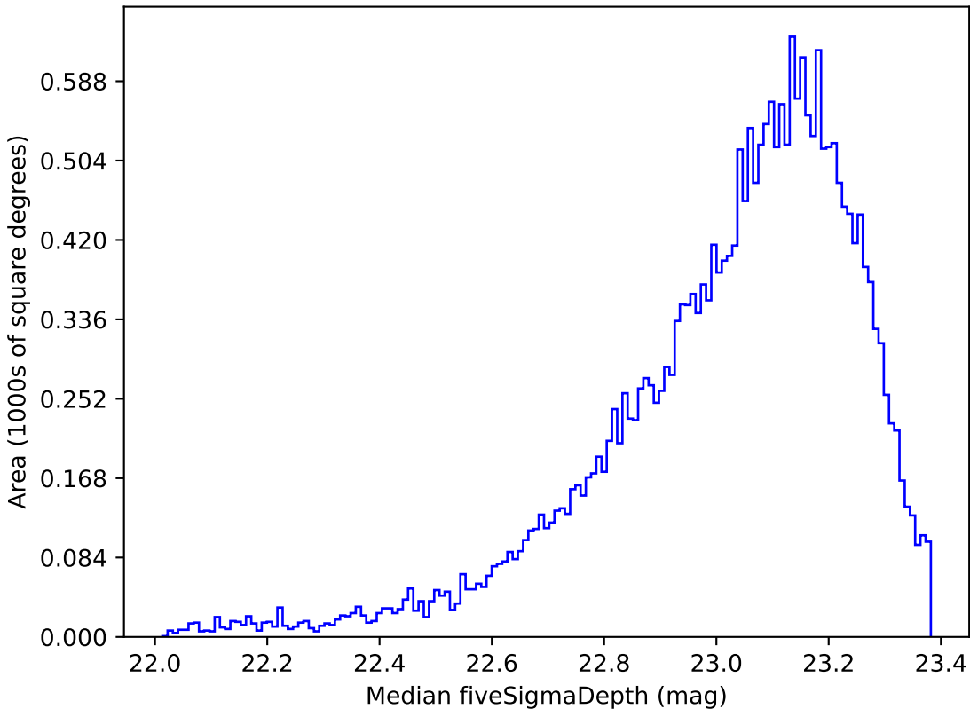
no_high_blob_v3.3_10yrs Yr 1 z band: Median fiveSigmaDepth
