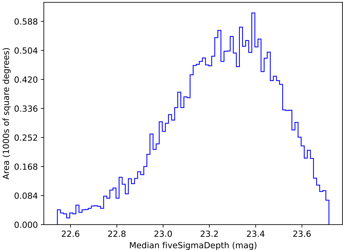
no_high_blob_v3.3_10yrs Yr 1 u band: Median fiveSigmaDepth
