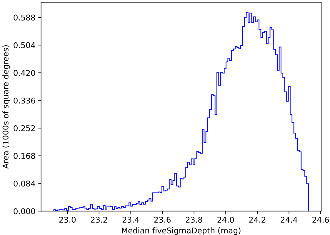
no_high_blob_v3.3_10yrs Yr 1 r band: Median fiveSigmaDepth
