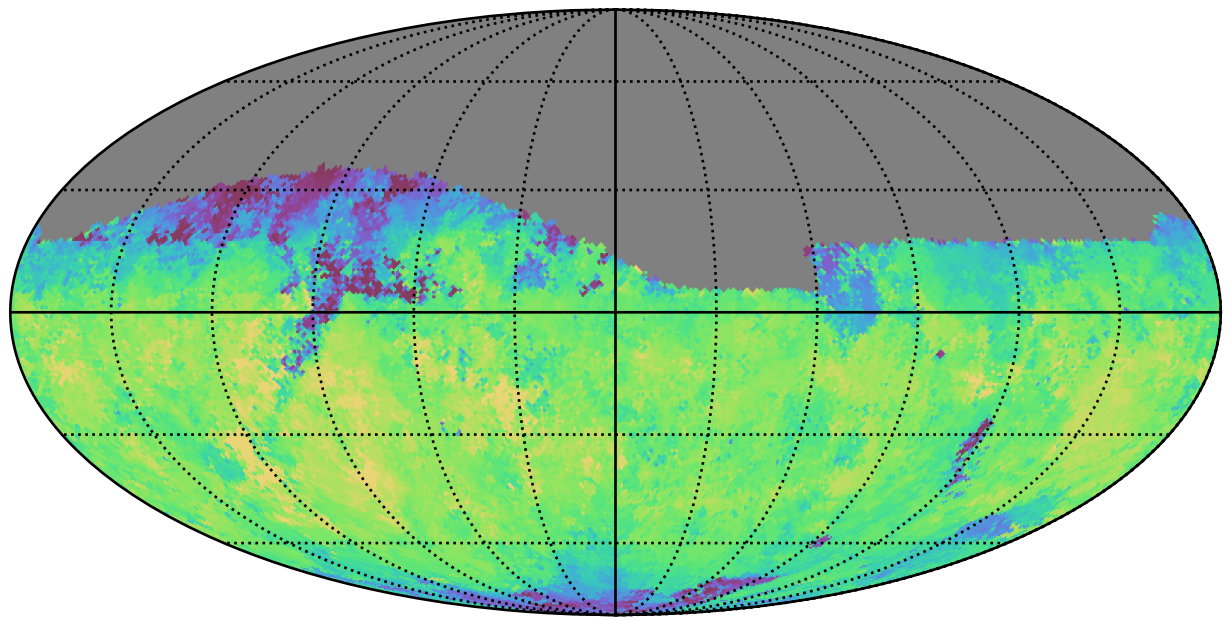
no_high_blob_v3.3_10yrs Yr 1 i band: Median fiveSigmaDepth
