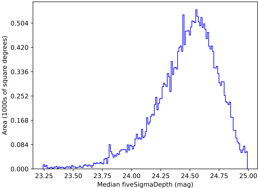
no_high_blob_v3.3_10yrs Yr 1 g band: Median fiveSigmaDepth
