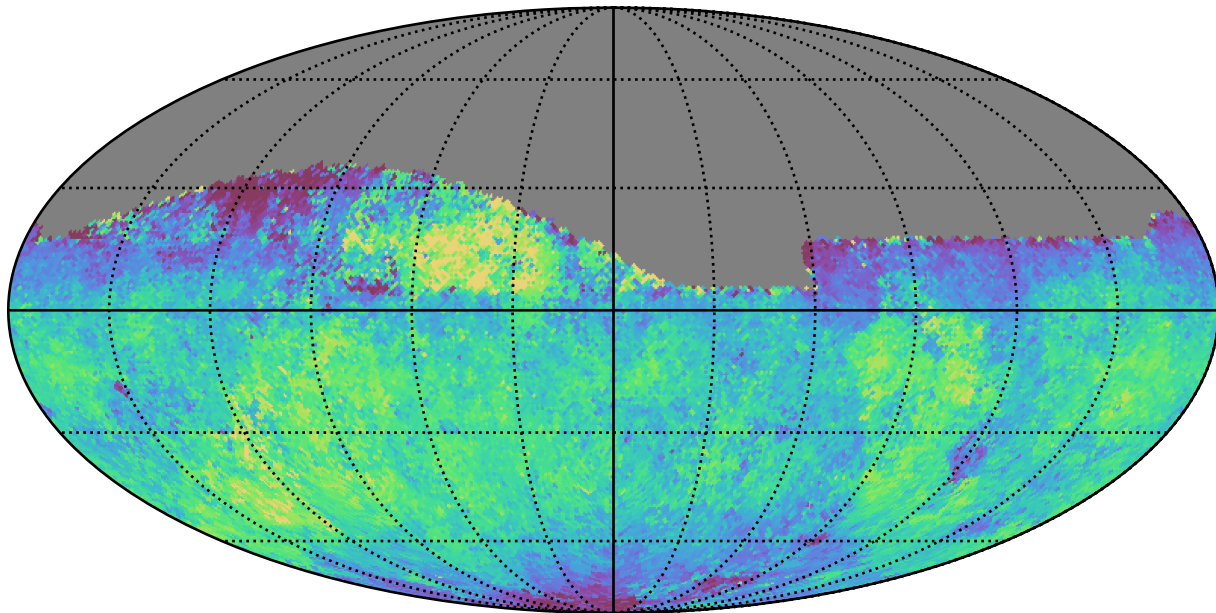
no_high_blob_v3.3_10yrs Yr 1 all bands: Median fiveSigmaDepth
