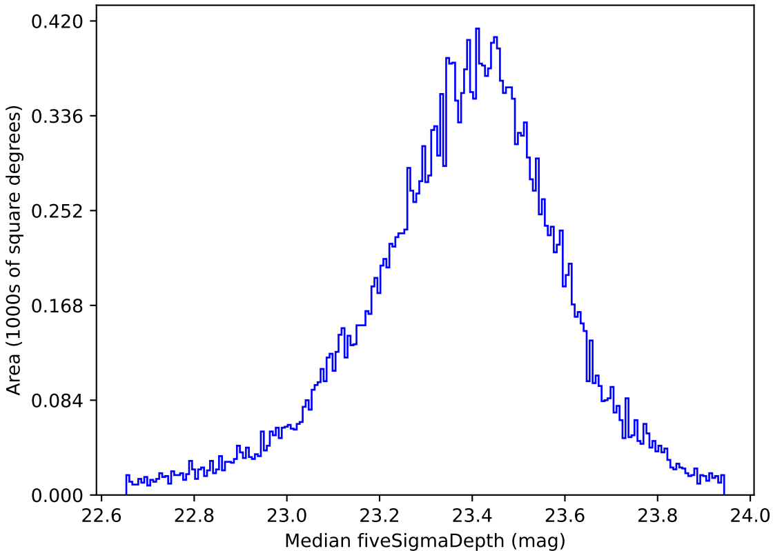
no_high_blob_v3.3_10yrs Yr 1 all bands: Median fiveSigmaDepth
