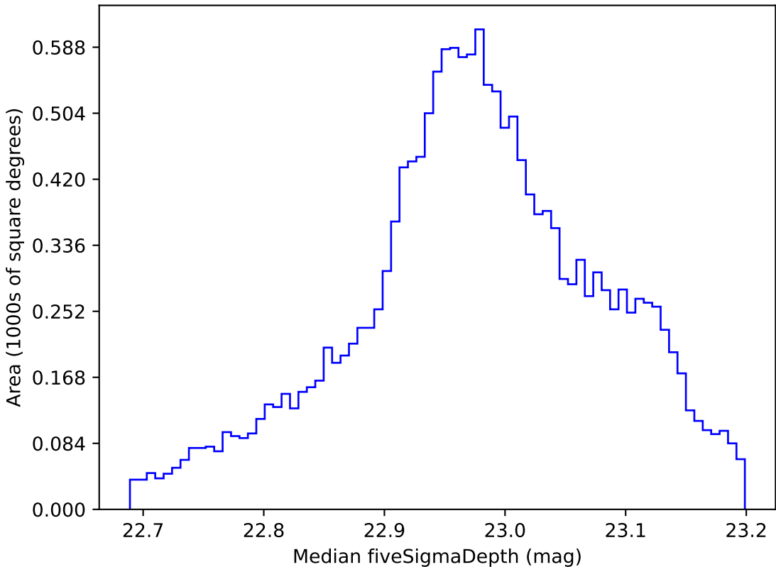
no_high_blob_v3.3_10yrs WFD z band: Median fiveSigmaDepth
