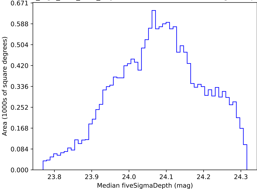
no_high_blob_v3.3_10yrs WFD r band: Median fiveSigmaDepth
