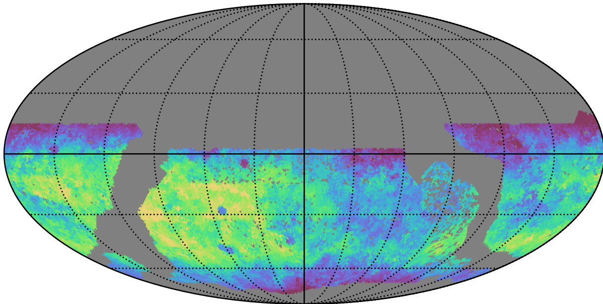
no_high_blob_v3.3_10yrs WFD g band: Median fiveSigmaDepth
