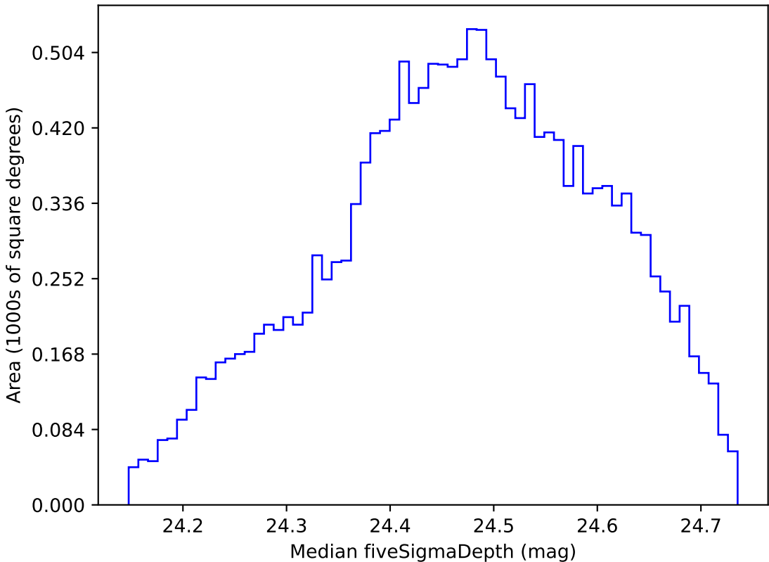
no_high_blob_v3.3_10yrs WFD g band: Median fiveSigmaDepth
