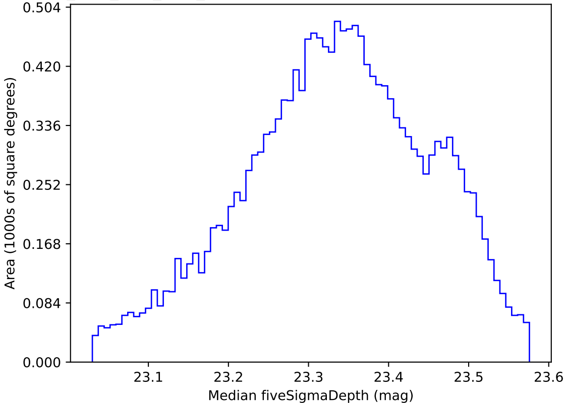
no_high_blob_v3.3_10yrs WFD all bands: Median fiveSigmaDepth
