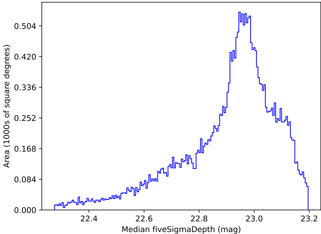
no_high_blob_v3.3_10yrs All sky z band: Median fiveSigmaDepth
