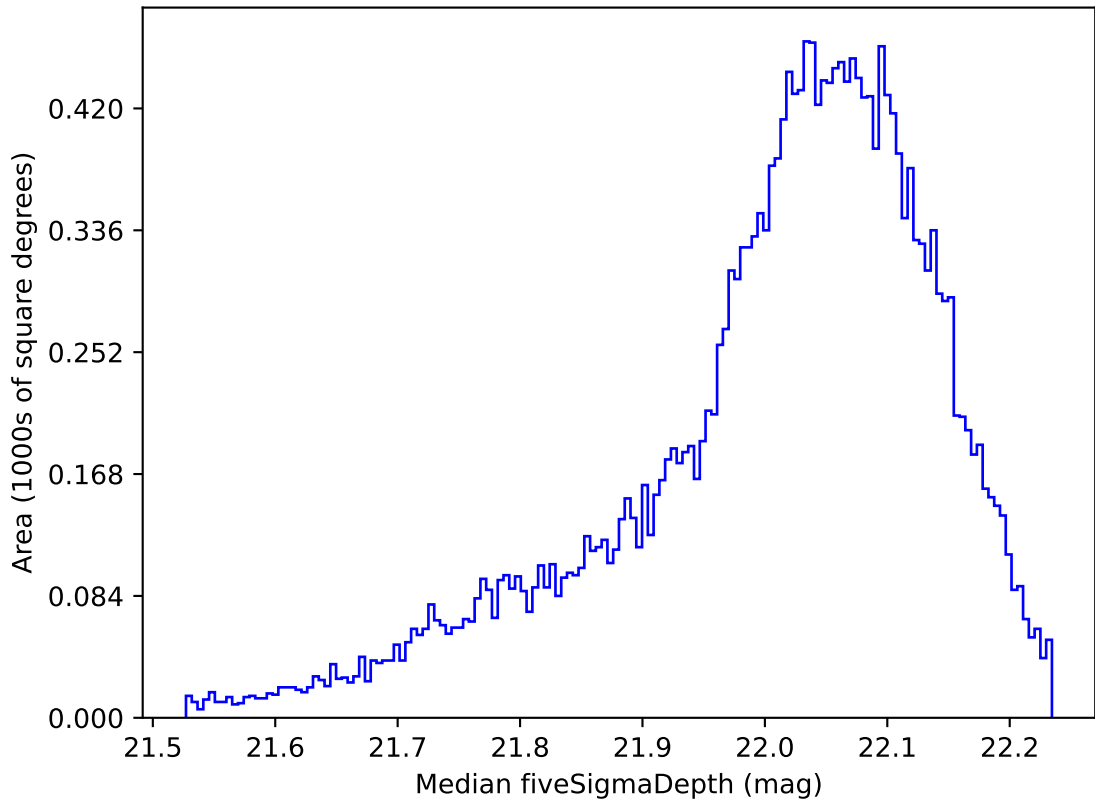
no_high_blob_v3.3_10yrs All sky y band: Median fiveSigmaDepth
