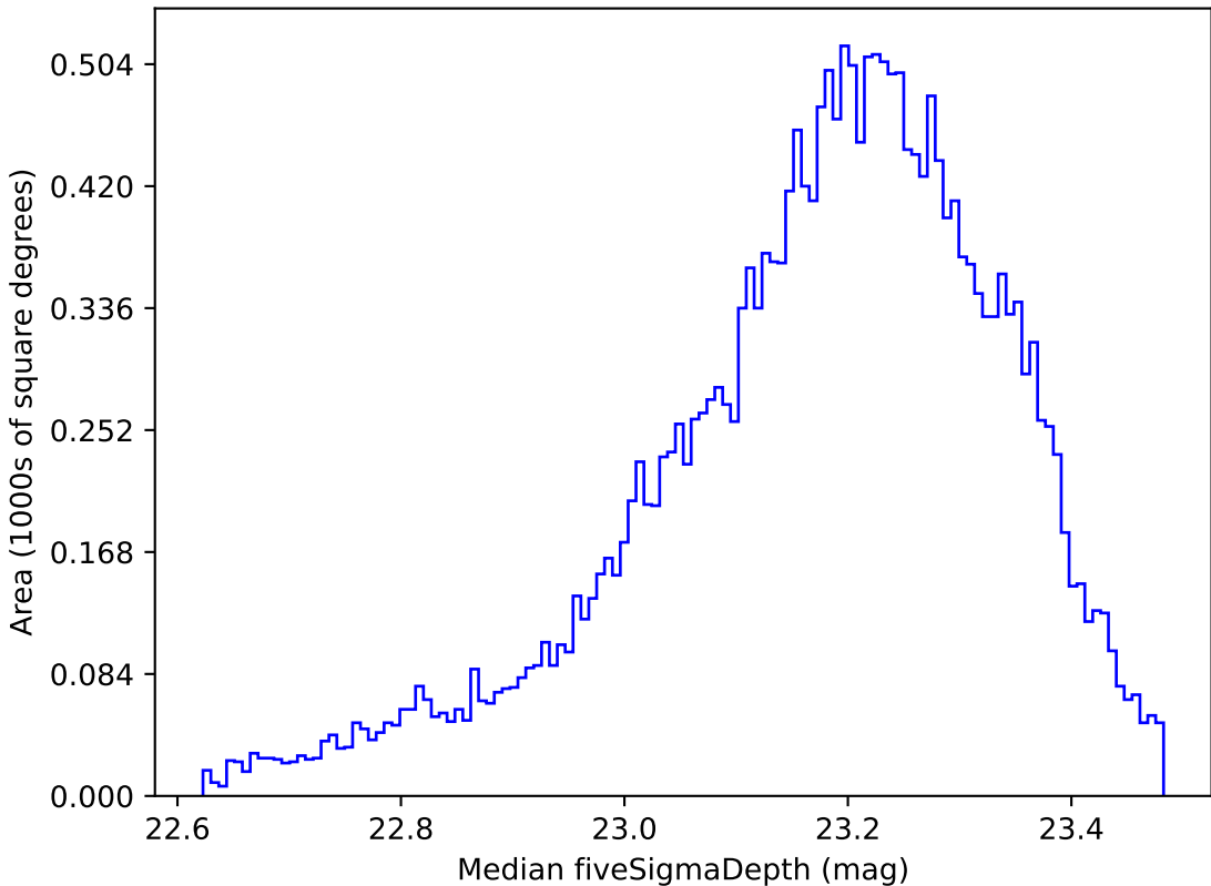
no_high_blob_v3.3_10yrs All sky u band: Median fiveSigmaDepth
