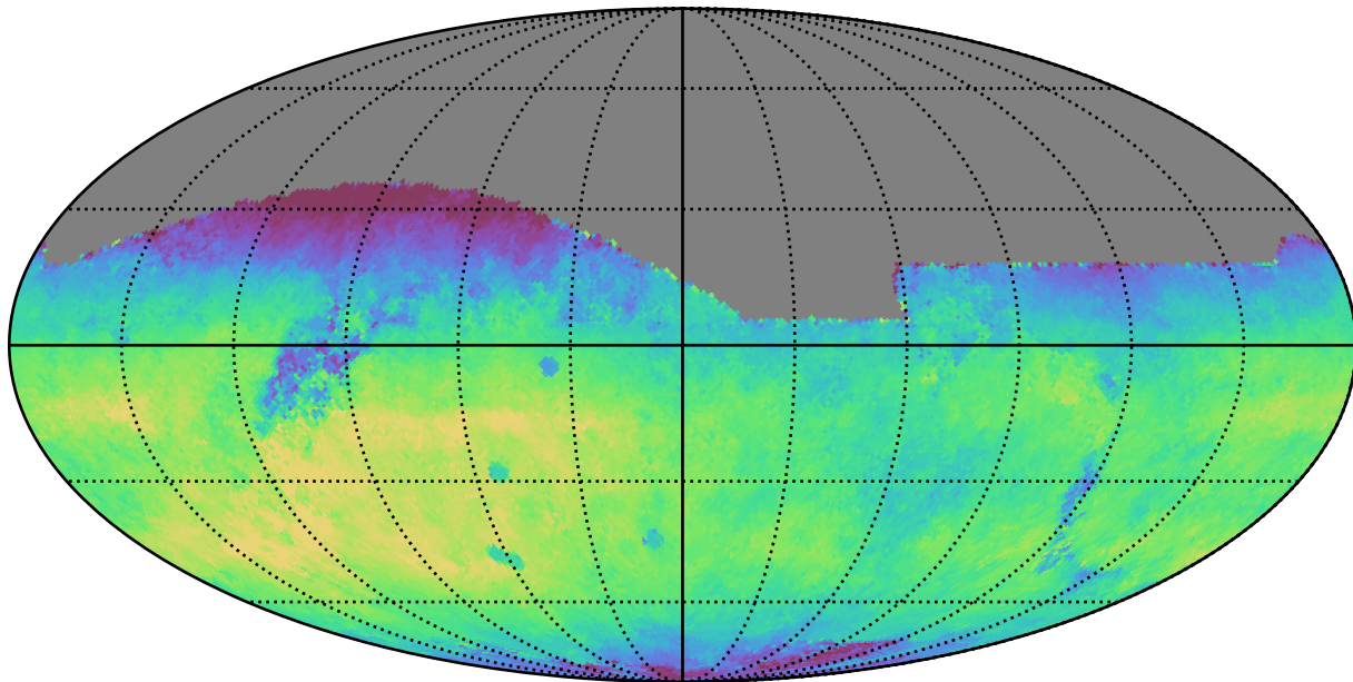
no_high_blob_v3.3_10yrs All sky r band: Median fiveSigmaDepth
