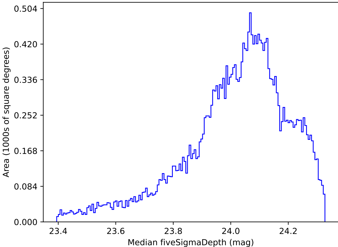
no_high_blob_v3.3_10yrs All sky r band: Median fiveSigmaDepth
