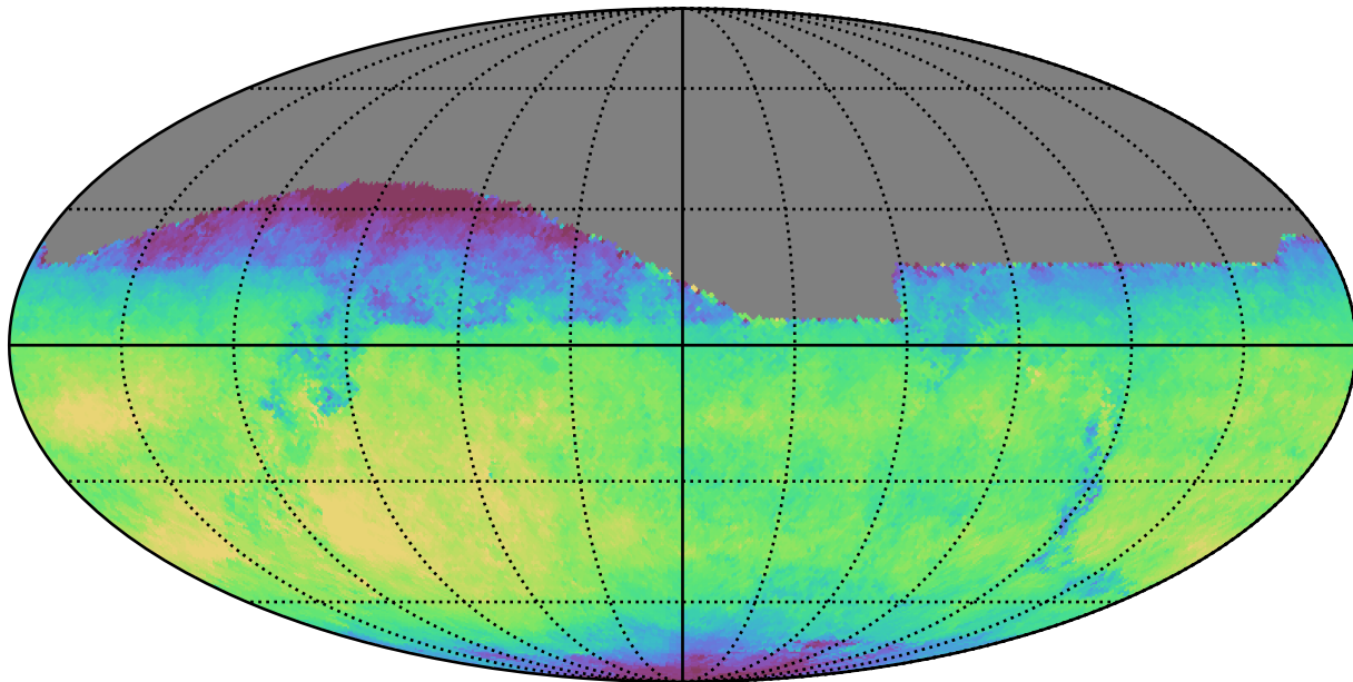
no_high_blob_v3.3_10yrs All sky i band: Median fiveSigmaDepth
