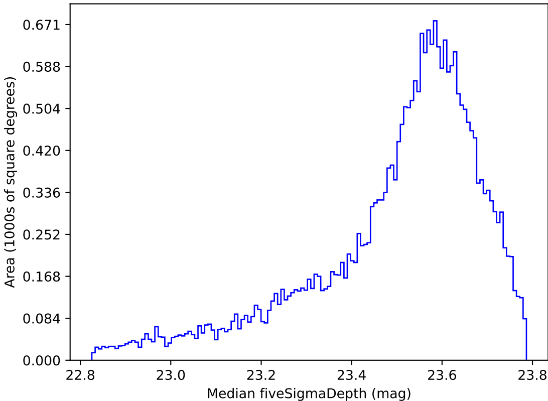
no_high_blob_v3.3_10yrs All sky i band: Median fiveSigmaDepth
