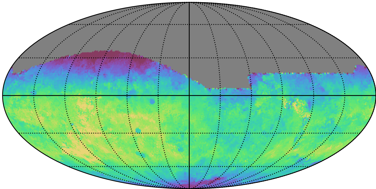
no_high_blob_v3.3_10yrs All sky g band: Median fiveSigmaDepth
