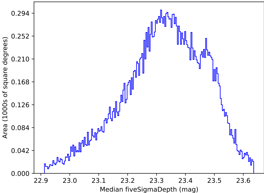
no_high_blob_v3.3_10yrs All sky all bands: Median fiveSigmaDepth
