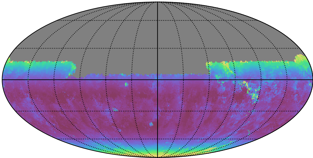
no_high_blob_v3.3_10yrs Yr 1 y band: Median airmass
