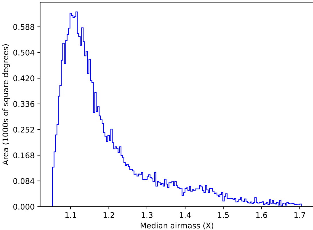
no_high_blob_v3.3_10yrs Yr 1 y band: Median airmass
