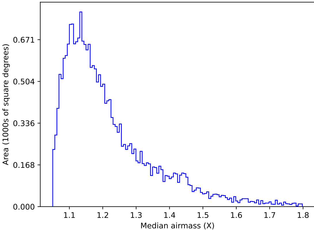
no_high_blob_v3.3_10yrs Yr 1 u band: Median airmass
