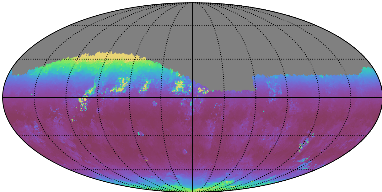
no_high_blob_v3.3_10yrs Yr 1 r band: Median airmass
