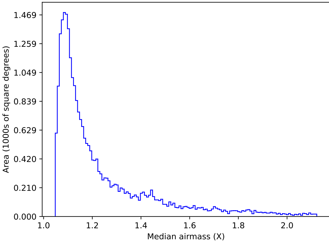
no_high_blob_v3.3_10yrs Yr 1 r band: Median airmass
