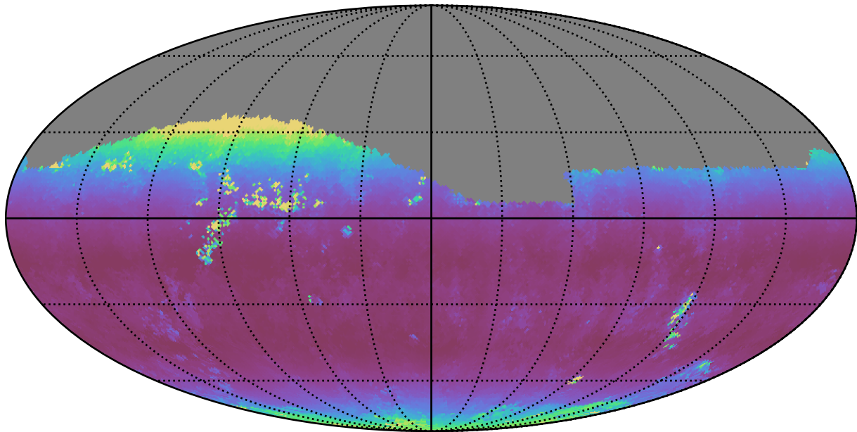
no_high_blob_v3.3_10yrs Yr 1 i band: Median airmass
