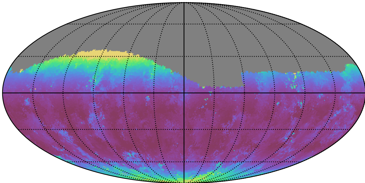
no_high_blob_v3.3_10yrs Yr 1 g band: Median airmass
