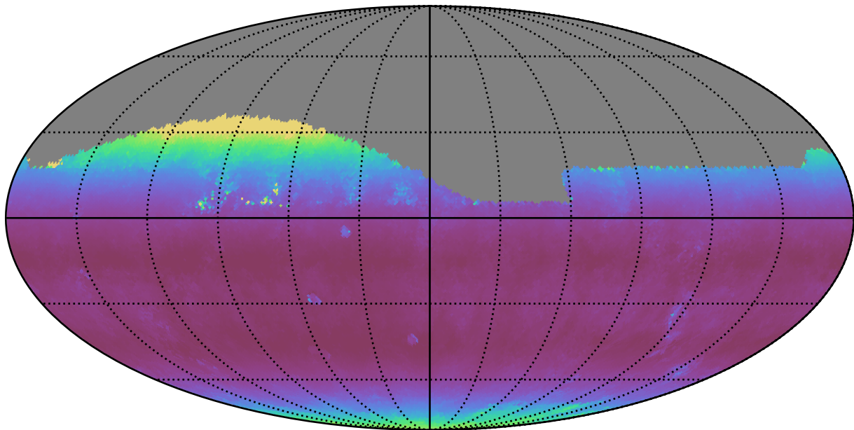
no_high_blob_v3.3_10yrs Yr 1 all bands: Median airmass
