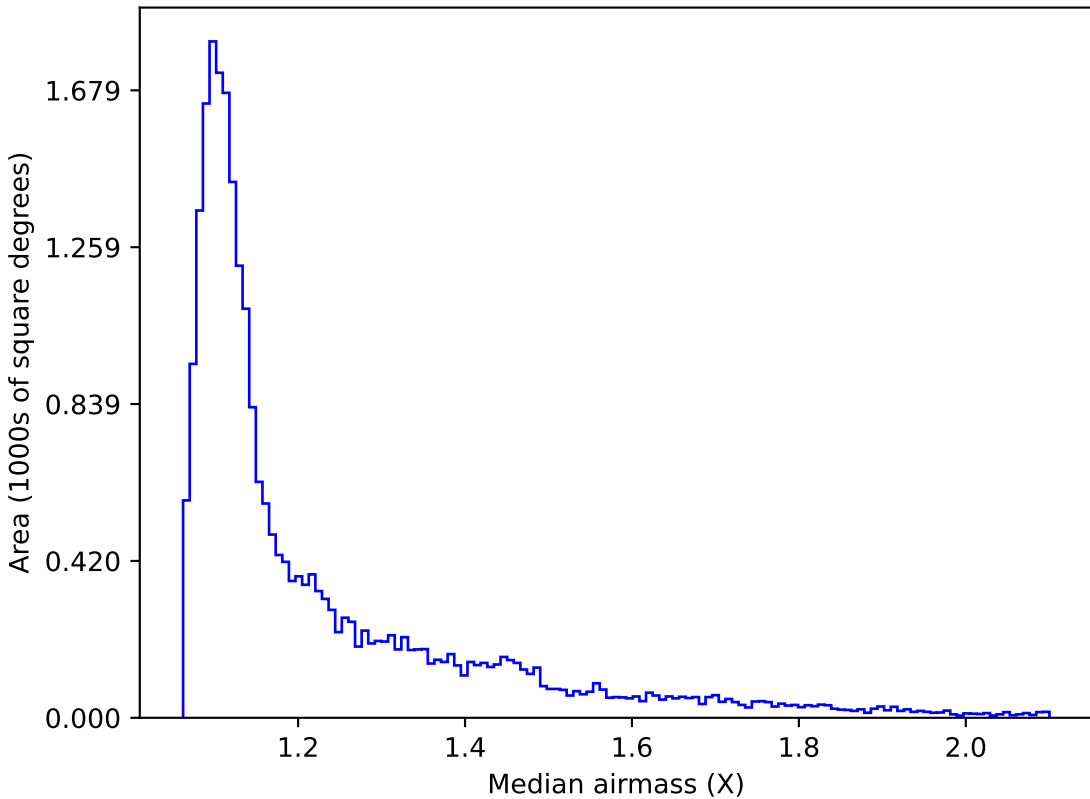
no_high_blob_v3.3_10yrs Yr 1 all bands: Median airmass
