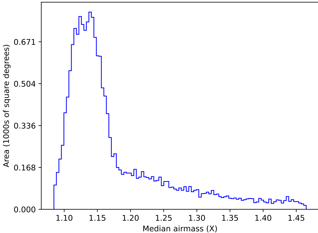
no_high_blob_v3.3_10yrs WFD z band: Median airmass
