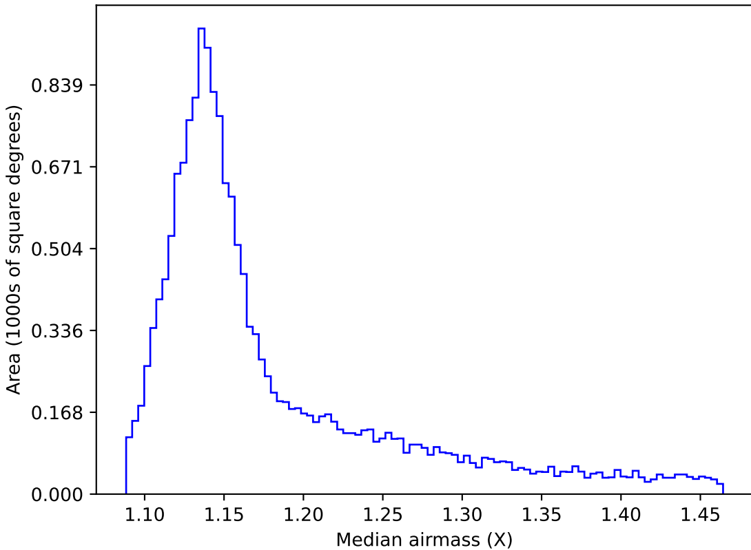
no_high_blob_v3.3_10yrs WFD y band: Median airmass
