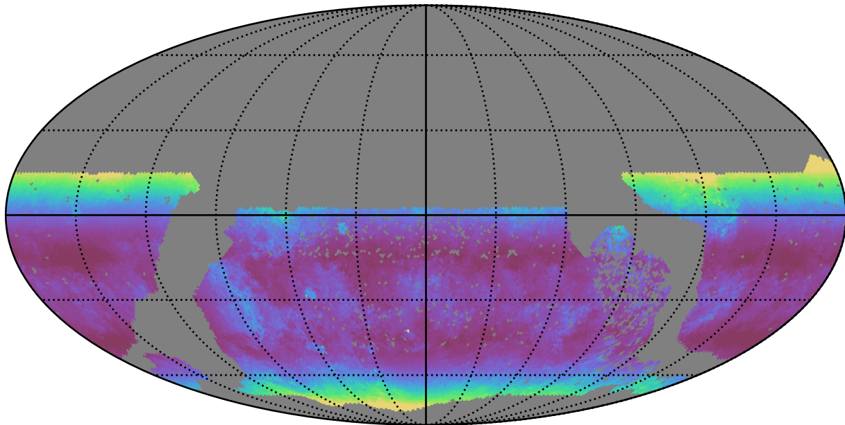
no_high_blob_v3.3_10yrs WFD u band: Median airmass
