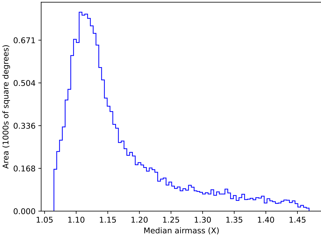
no_high_blob_v3.3_10yrs WFD u band: Median airmass
