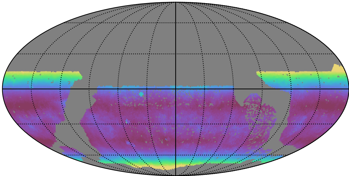
no_high_blob_v3.3_10yrs WFD i band: Median airmass
